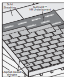
Asphalt based shingles
