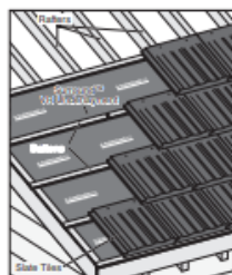
Slate over rafters and batten
