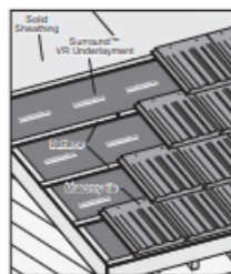
Masonry tiles over solid sheathing
